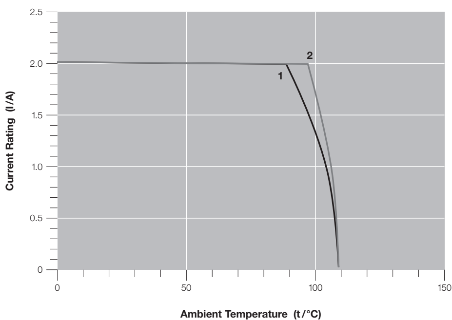
Derating Curve
