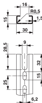
Dimensional drawing
