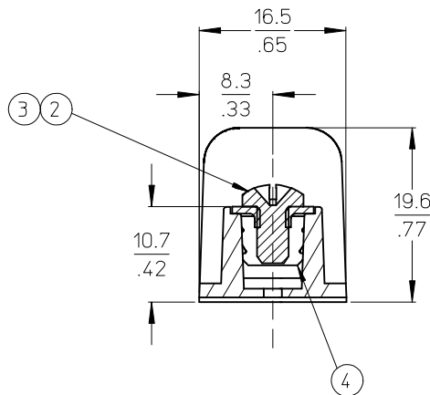
SECTION Z-Z
