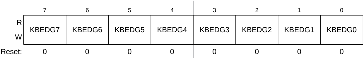
Figure 7-5. KBIx Edge Select Register
