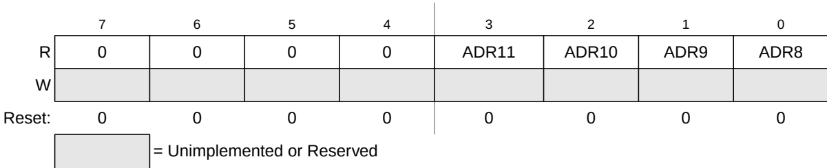
Figure 15-6. Data Result High Register (ADCRH)
