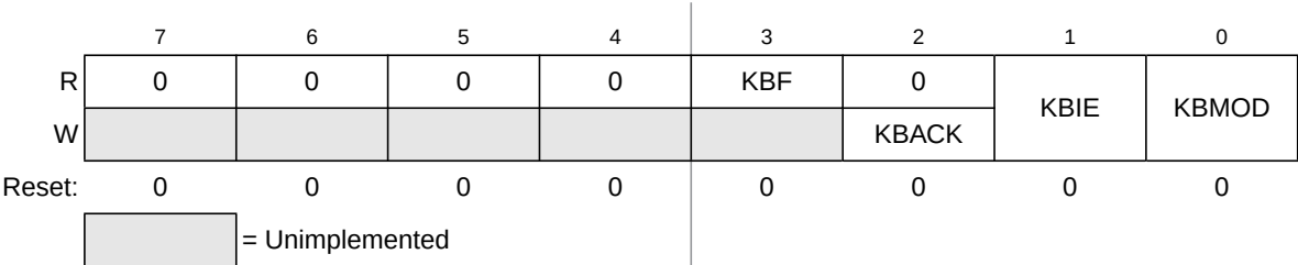
Figure 7-3. KBIx Status and Control Register
