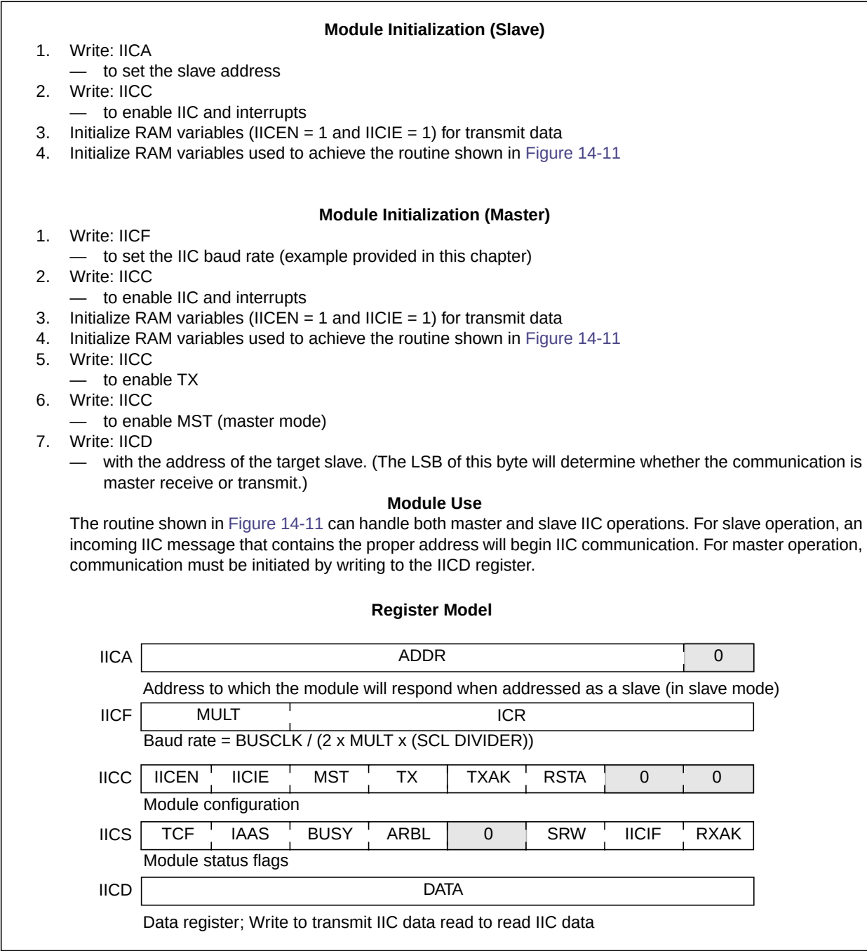
Figure 14-10. IIC Module Quick Start
