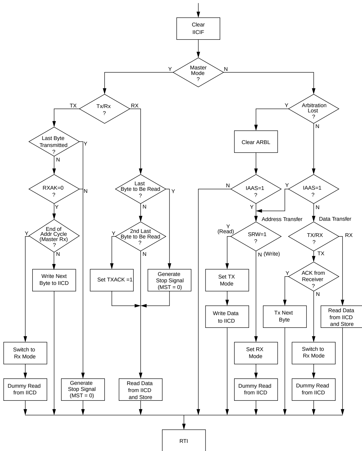
Figure 14-11. Typical IIC Interrupt Routine
