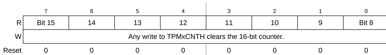
Figure 11-4. Timer x Counter Register High (TPMxCNTH)
