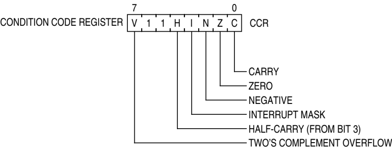
Figure 8-2. Condition Code Register
