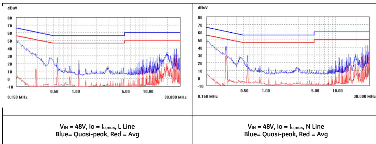
Figure 26. EMC Considerations.
