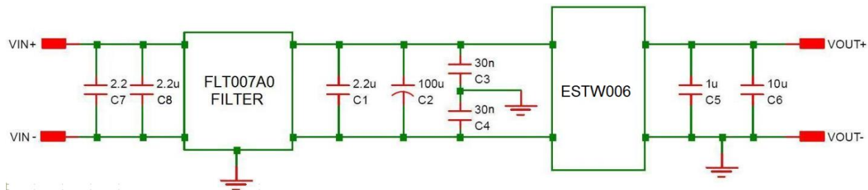
Figure 26. EMC Considerations.
