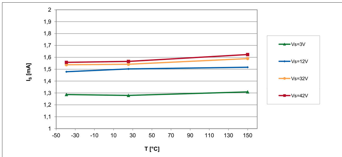
Figure 6-3 Supply Current of the TLE4964-2K over Temperature
