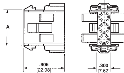
Cap Front
