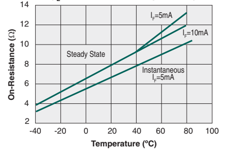
Typical On-Resistance vs. Temperature ( I_L=Max\ Rated\ @\ Temperature )
