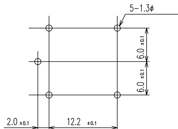
4. DRILLING DIAGRAM
