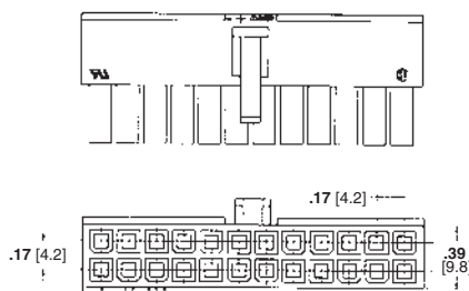
Receptacle Housing
