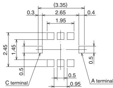
Metal mask dimensions
