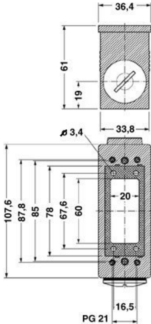
Dimensional drawing
