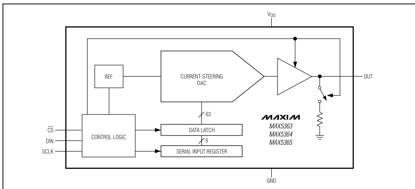
Figure 1. Functional Diagram
