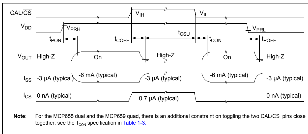
FIGURE 1-1: Timing Diagram.
