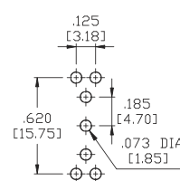
P.C.MOUNTING
