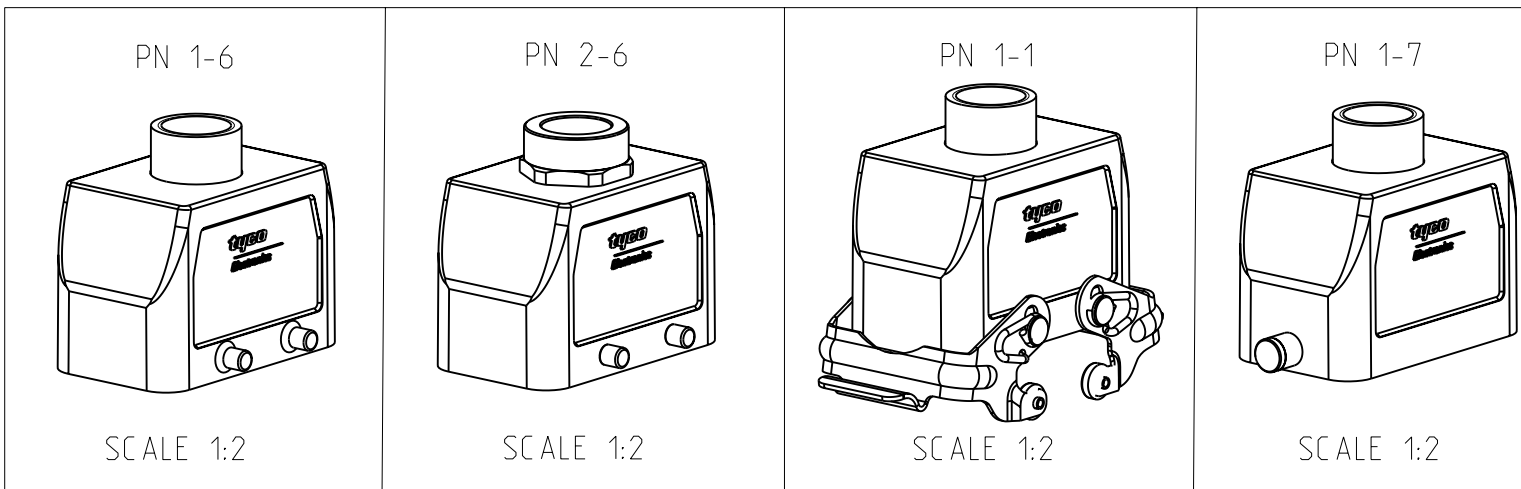
1 O-Ring PG16 Neoprene - Black 8 1 6-KI-Adaptor PG16 Brass Nickel plated Blue 7 1 1 1 Adaptor round PG16 Brass Nickel plated Blue 6 2 LB-Slide spool Steel Zinc plated - 5 2 VS-Side clip Steel Zinc plated Blue 4 4 VS-Clip bolt Stainless steel Blank - 3 1 Hood HB.10 Aluminium Aluminium oxide Black 2 1 1 1 Hood HB.10 Aluminium - Grey 1 1-7 1-12 6-1 6-6 DESCRIPTION MATERIAL SURFACE COLOR ITEM NO NOTES ORDERING TEXT HB.10.STO.1.16.Z HB-K.10.STO.1.16.Z HB.10.STO-VS.1.16.Z HB.10.STO-GR.1.16.Z
