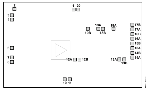
Figure 2. Pad Configuration
