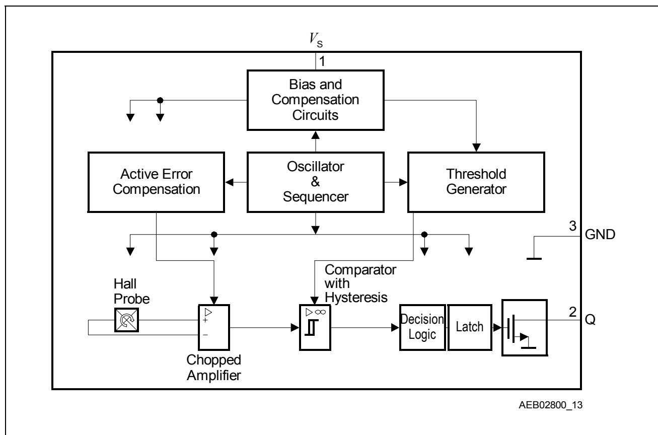
Figure 2 Block Diagram
