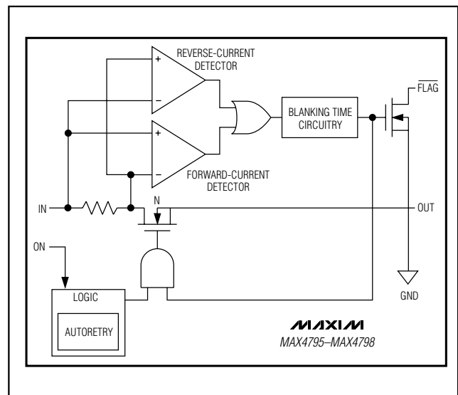
Figure 1. Functional Diagram
