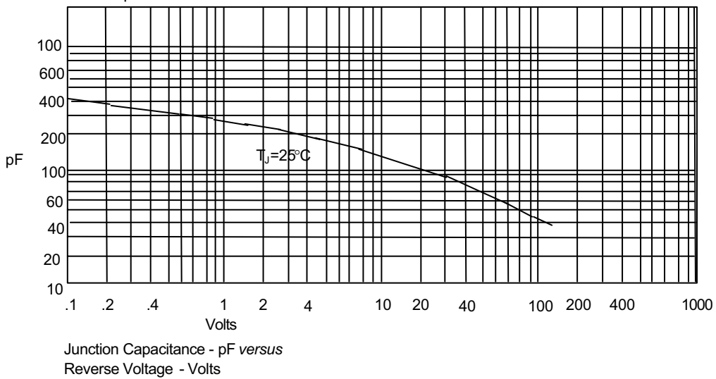
Figure 3 Junction Capacitance
