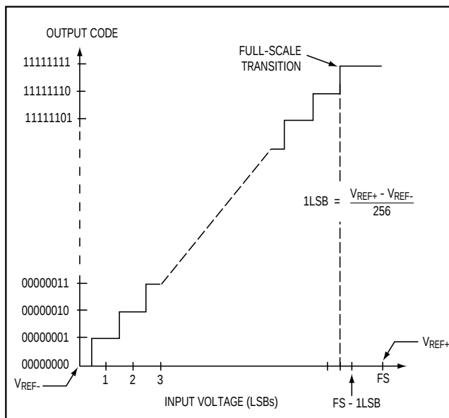
Figure 10. Transfer Function
