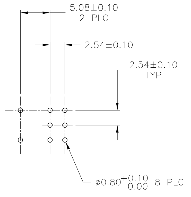
RECOMENDED P.C. HOLE LAYOUT DOUBLE POLE
