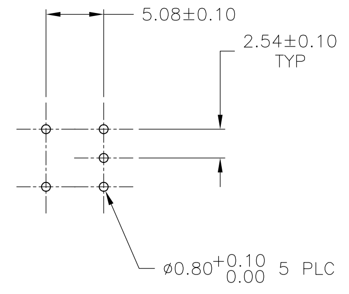
RECOMENDED P.C. HOLE LAYOUT SINGLE POLE
