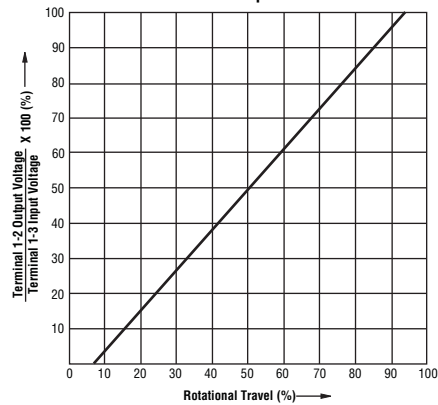
B0 Taper
