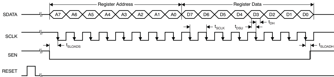
Figure 13. Serial Interface Timing
