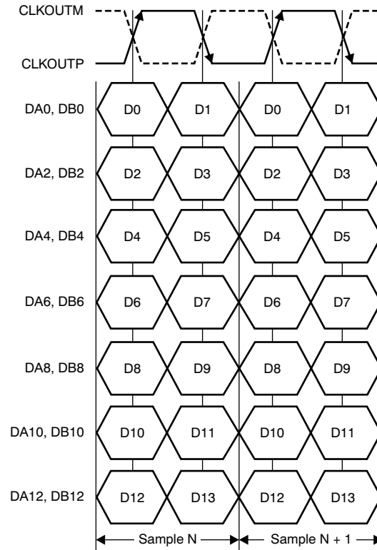
Figure 10. ADS4246/45/42 LVDS Interface Timing Diagram
