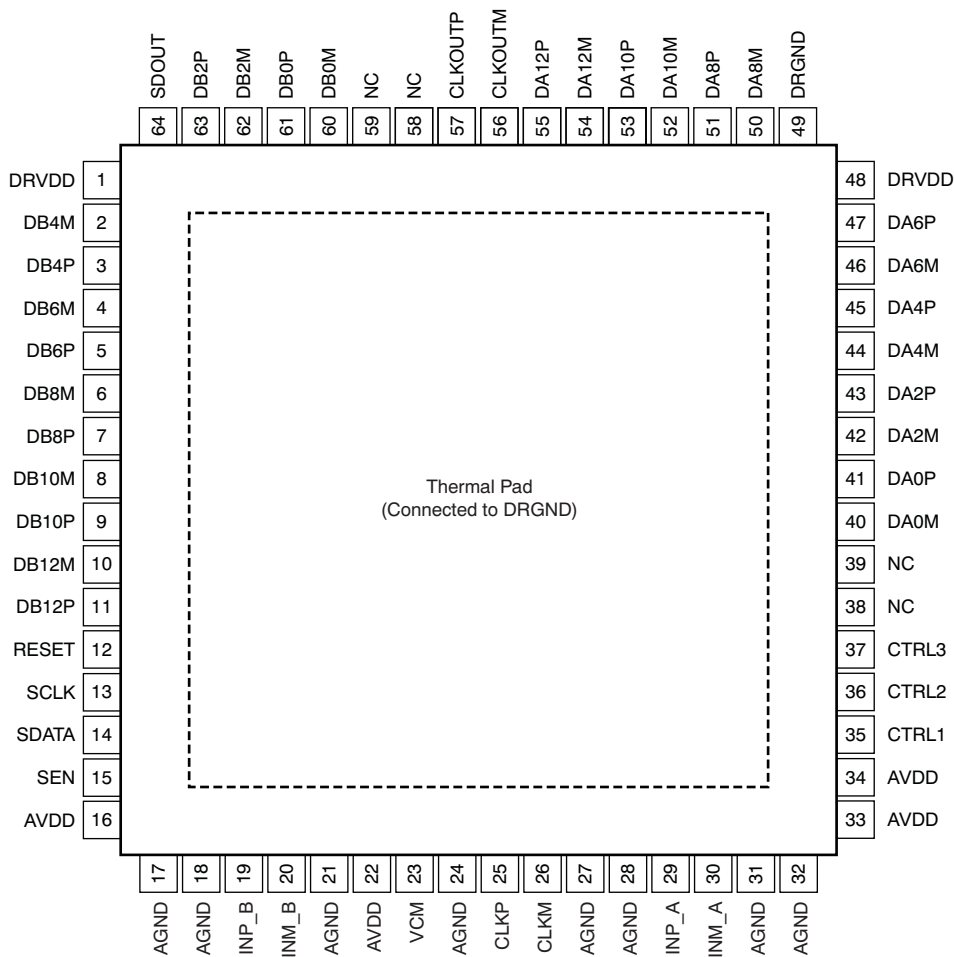
Figure 2. ADS4246/ADS4245/ADS4242 LVDS Mode
