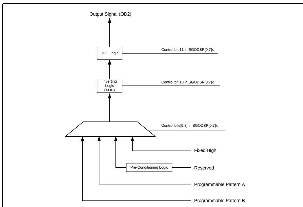
Figure 5-26. SGPIO Output OD2 Signal
