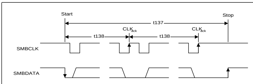
Figure 8-21. SMBus/SMLink Timeout
