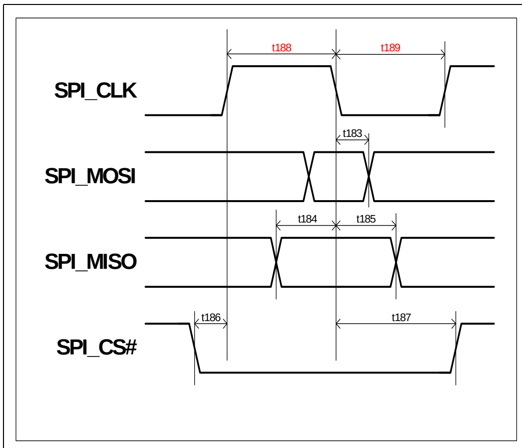
Figure 8-22. SPI Timings
