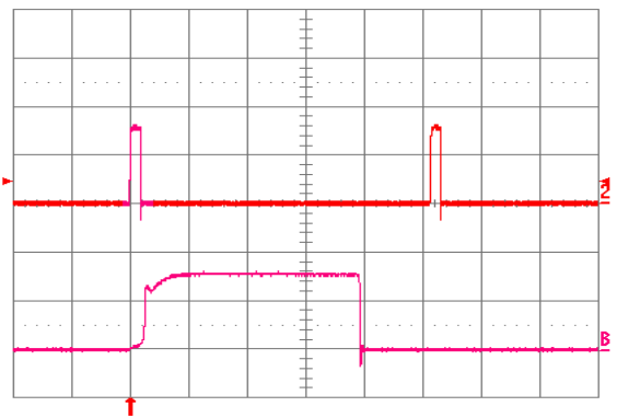
Fig. 17: Load current (top trace, 20 A/div, 20 ms/div) into a 10 m\Omega short circuit during restart, at V_{in} = 48 V. Bottom trace (20 A/div, 1 ms/div) is an expansion of the on-time portion of the top trace.
