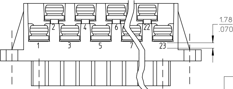
OPTIONAL 10A IMPRINTING (ODD CIRCUIT CONFIGURATION SHOWN)
