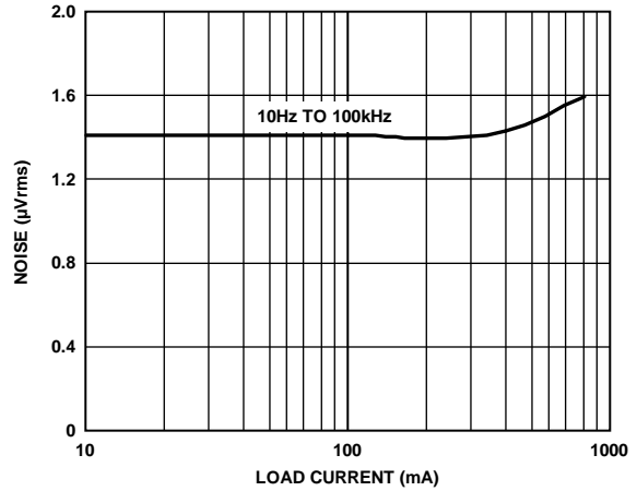
Figure 33. RMS Output Noise vs. Load Current ( I_{LOAD} ), 10 Hz to 100 kHz, ADM7151-02, V_{OUT} = 4V
