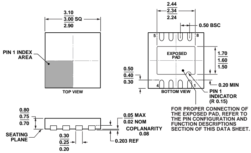
Figure 71. 8-Lead Lead Frame Chip Scale Package [LFCSP_WD] 3 mm × 3 mm Body, Very Very Thin, Dual Lead (CP-8-11)
