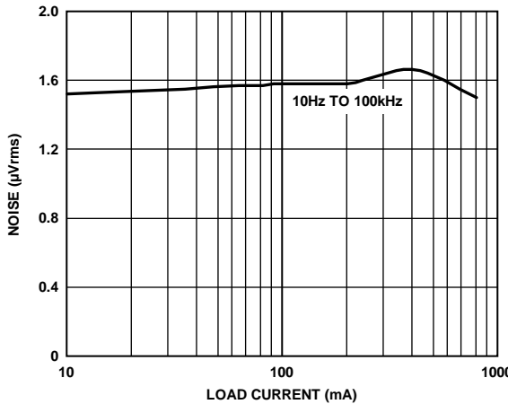
Figure 31. RMS Output Noise vs. Load Current ( I_{LOAD} ), 10 Hz to 100 kHz, ADM7151-04, V_{OUT} = 5V
