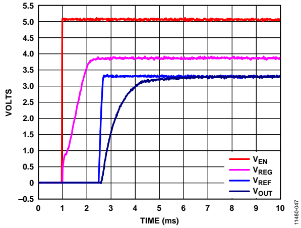
Figure 47. V_{OUT} , V_{REF} , V_{REG} Start-Up Times After V_{EN} Rising, V_{OUT} = 3.3V , V_{IN} = 5V
