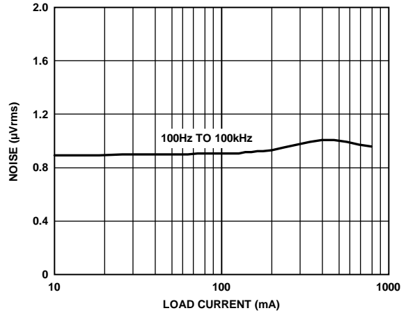
Figure 32. RMS Output Noise vs. Load Current ( I_{LOAD} ), 100 Hz to 100 kHz, ADM7151-04, V_{OUT} = 5V
