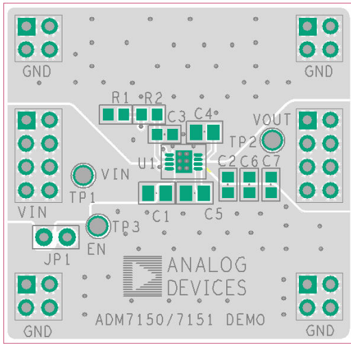
Figure 69. Example 8-Lead LFCSP PCB Layout
