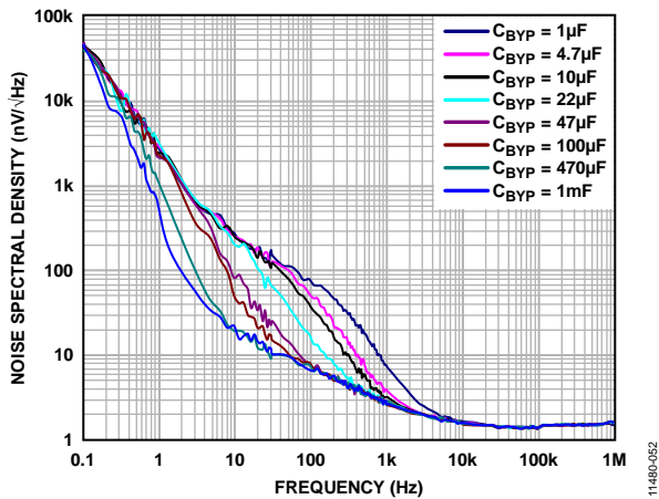
Figure 52. Noise Spectral Density vs. Frequency, C BYP = 1 μF to 1 mF
