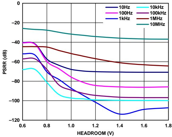
Figure 29. Power Supply Rejection Ratio (PSRR) vs. Headroom Voltage, ADM7151-04, V_{OUT} = 5V , 400 mA Load
