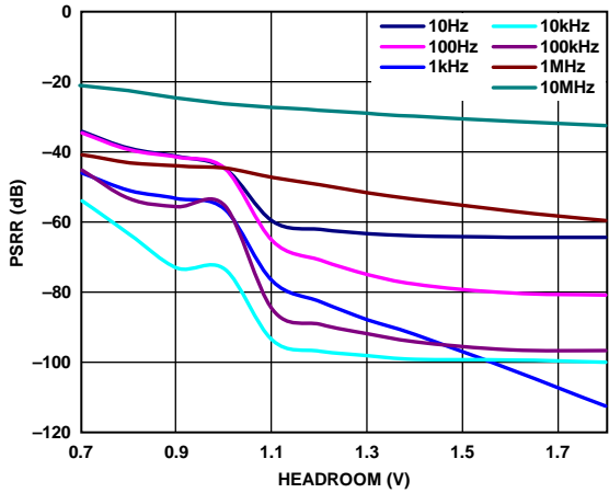
Figure 30. Power Supply Rejection Ratio (PSRR) vs. Headroom Voltage, ADM7151-04, V_{OUT} = 5V , 800 mA Load
