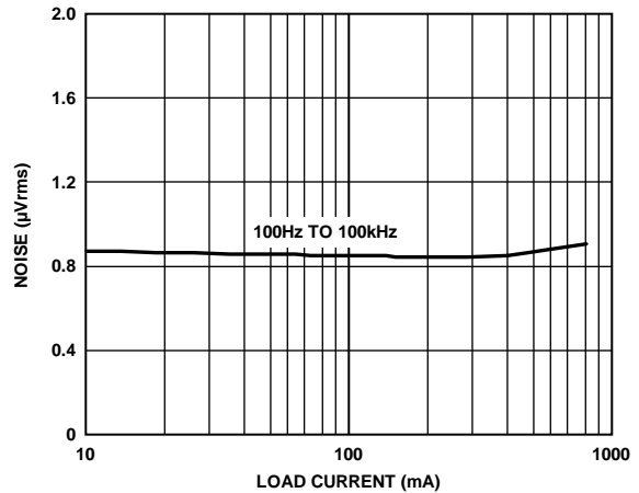
Figure 34. RMS Output Noise vs. Load Current ( I_{LOAD} ), 100 Hz to 100 kHz, ADM7151-02, V_{OUT} = 4V
