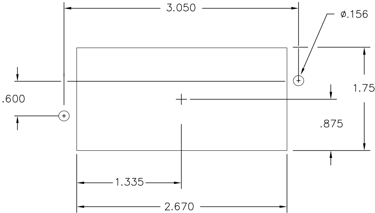
PIN PANEL MOUNT CUTOUT SCALE: NONE
