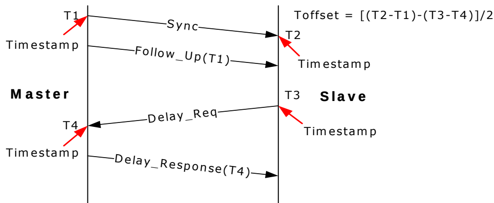
Figure 11-1. Sync flow and offset calculation
