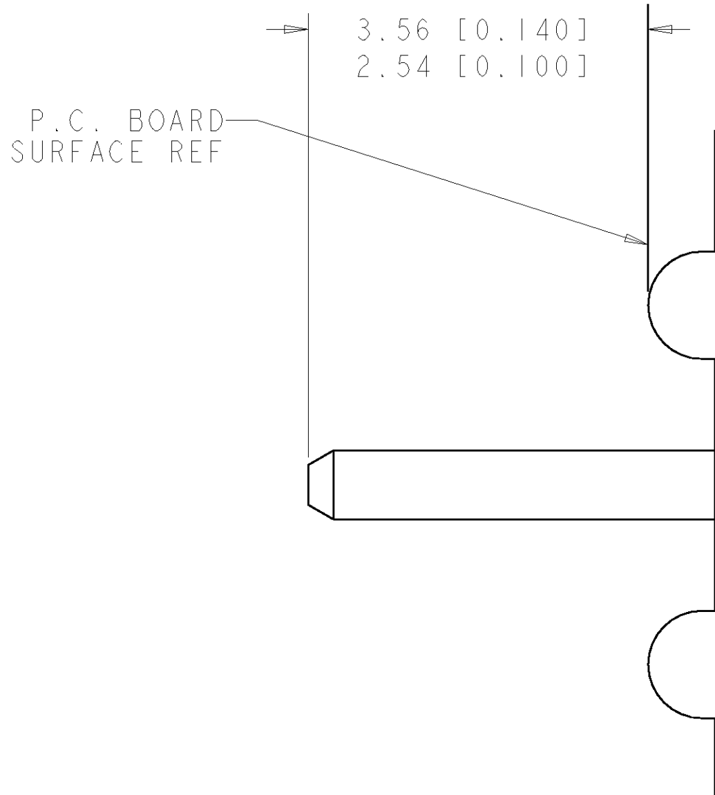
6. SOLDER PIN DETAIL SCALE 10:1
