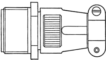
Cable connecting plug MS 3101E and F / CA 3101E Dimensions / sizes
