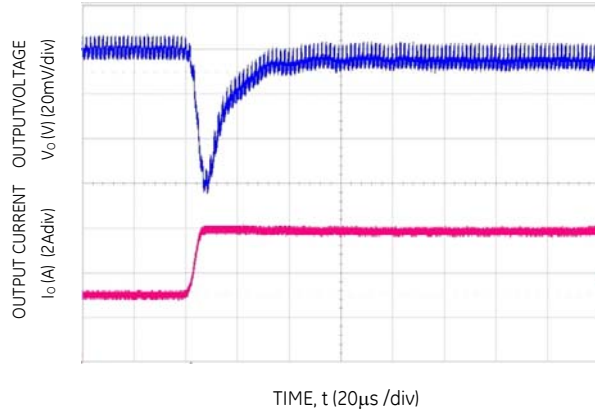
Figure 28. Transient Response to Dynamic Load Change from 50% to 100% at 12V in , C out -3x47µF, C Tune -178 & R Tune -3900pF
