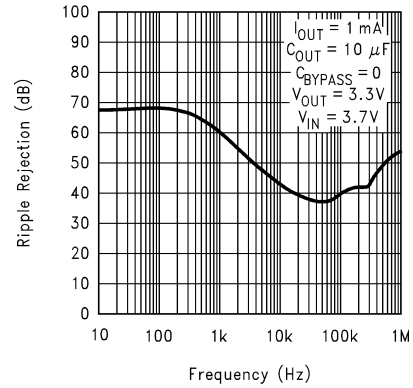
Figure 6-8. Ripple Rejection vs Frequency for Legacy Chip
