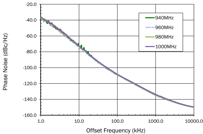
VCO Phase Noise versus Frequency +2.2V Supply
