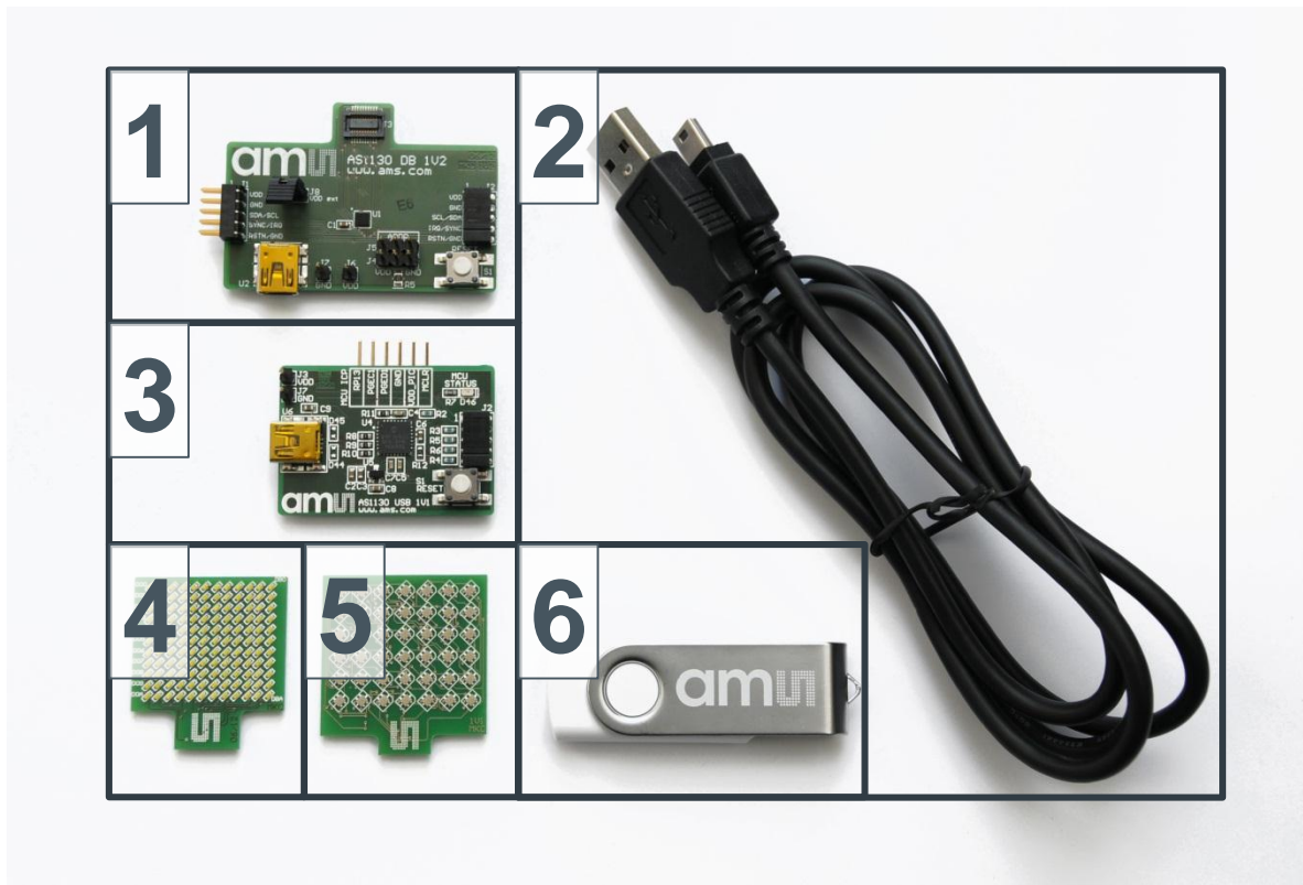
Figure 1: Kit Content
