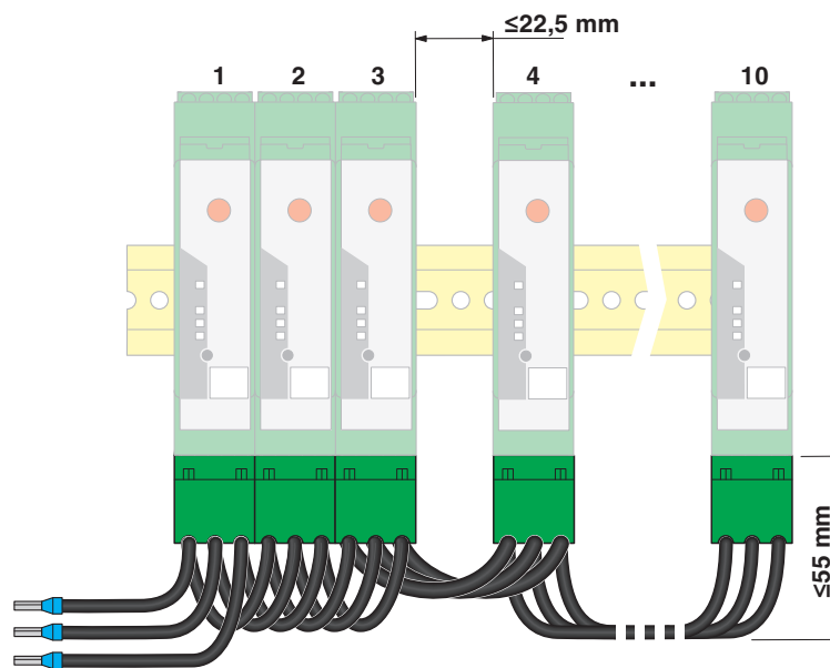
Application drawing
