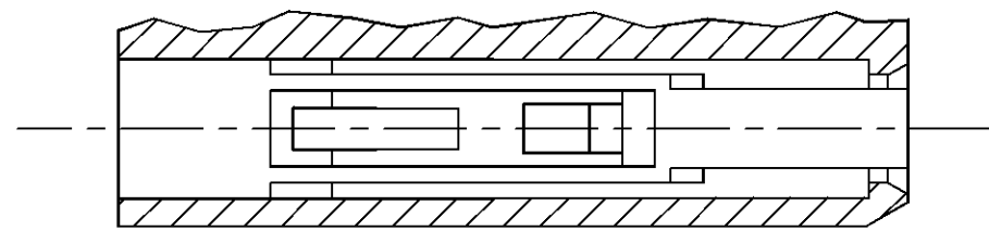
SECTION H-H
