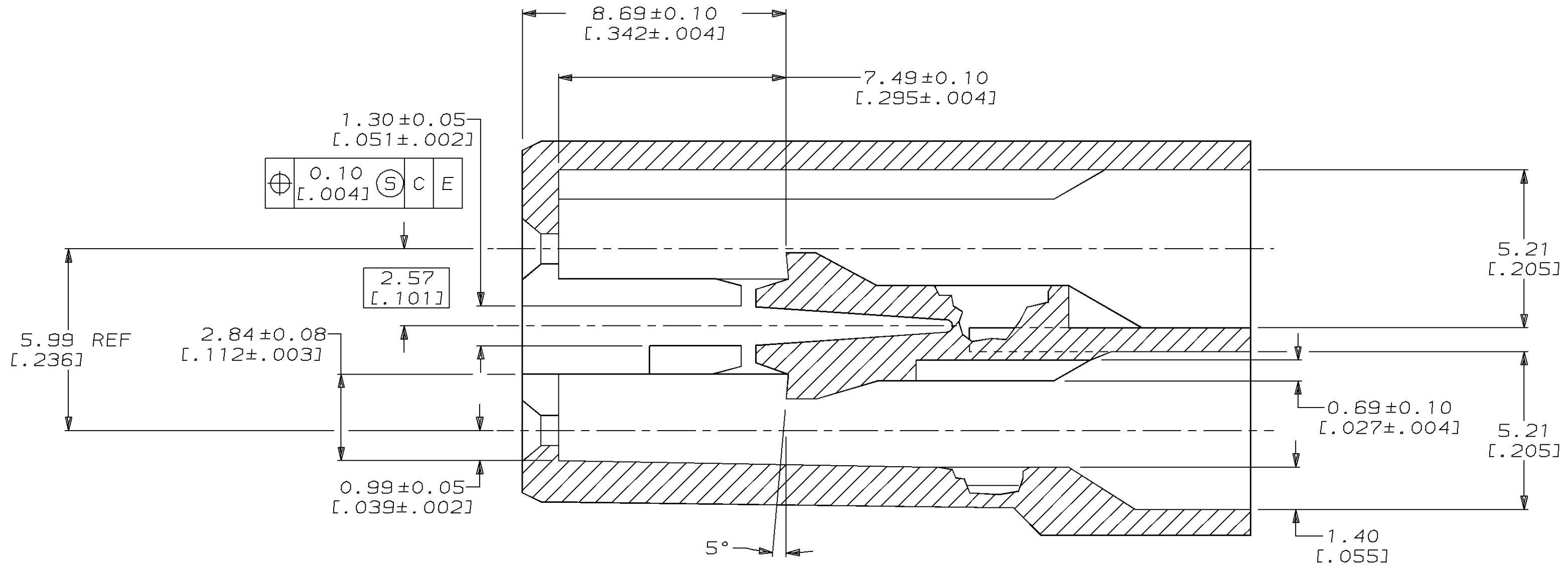
SECTION B-B SCALE 8:1
