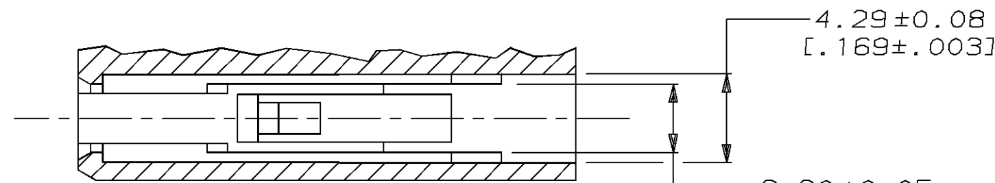
SECTION G-G
