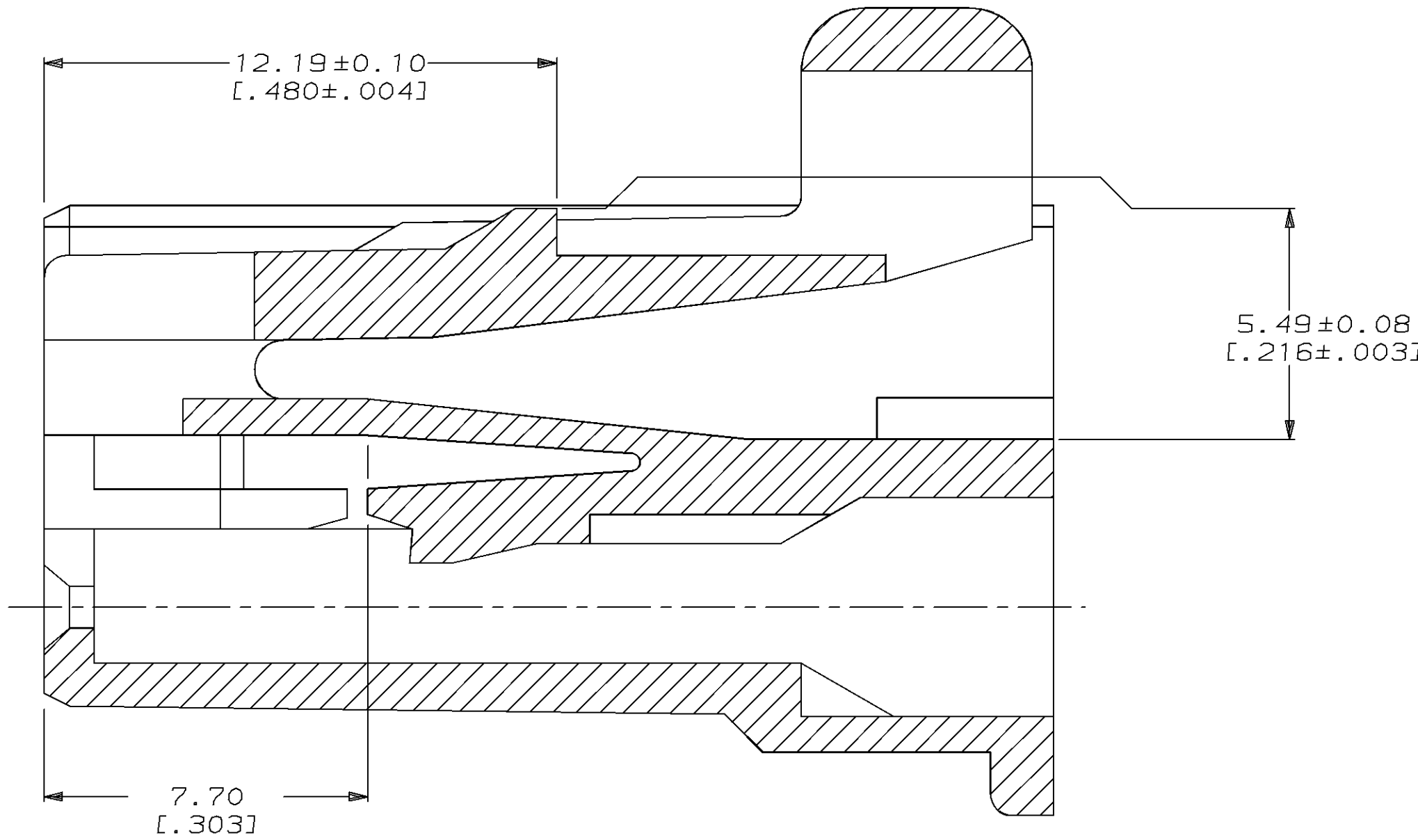
SECTION D-D SCALE 8:1
