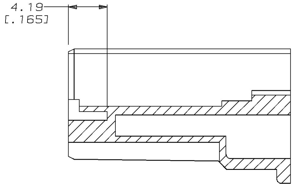
SECTION C-C
