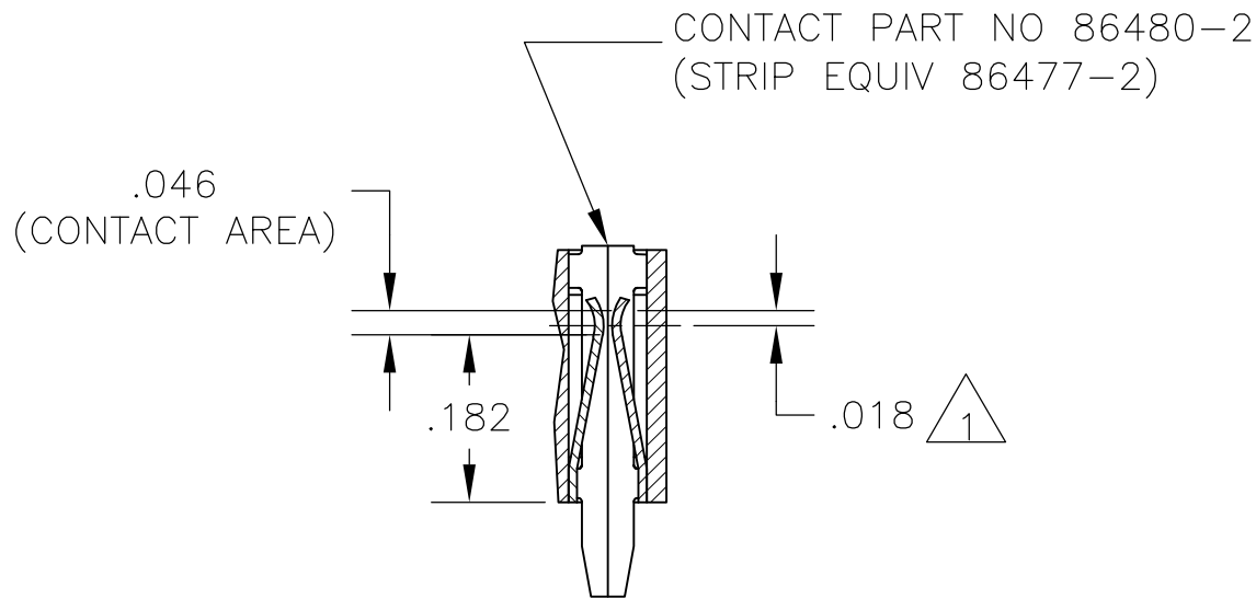
SECTION X-X
