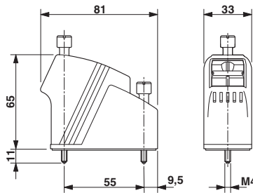
Dimensional drawing
