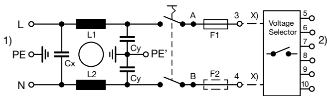
Standard version with fuseholder 1- or 2-pole
