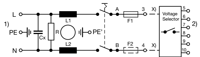
Medical version (M5) with fuseholder 2-pole
