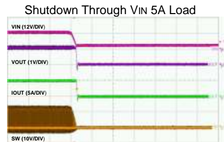
Time-500μs/div
