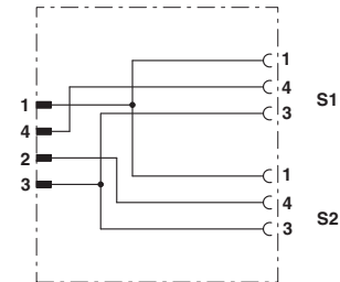
Contact assignment of the M8 Y distributor
