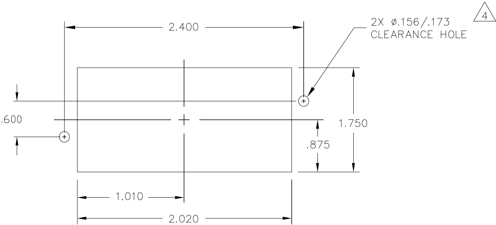
PIN PANEL MOUNT CUTOUT SCALE: NONE
