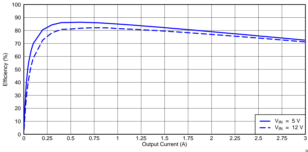
Figure 1. TPS54329EVM-056 Efficiency
