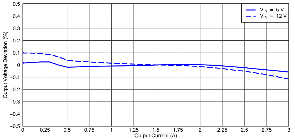
Figure 3. TPS54329EVM-056 Load Regulation, V_{IN} = 5V
