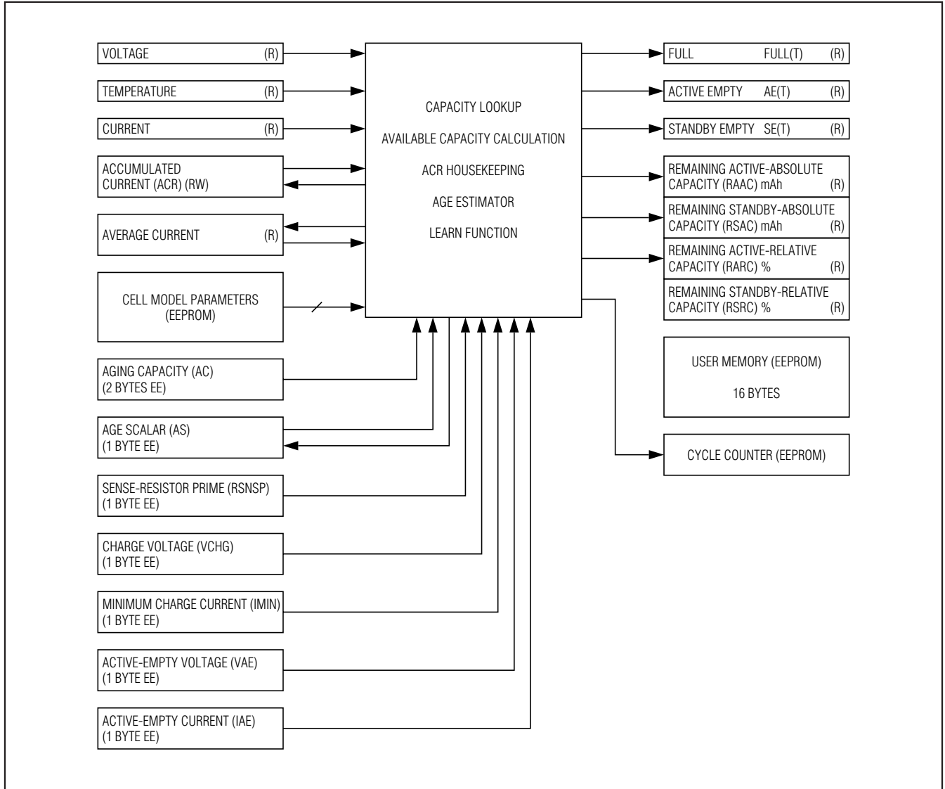
Figure 13. Top-Level Algorithm Diagram
