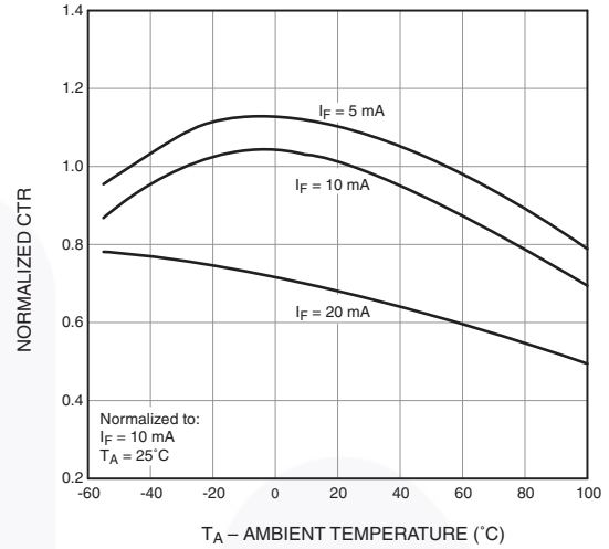
Figure 4. Normalized CTR vs. Ambient Temperature
