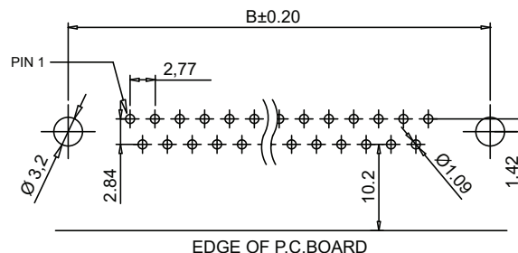
RECOMMENDED P.C.B LAYOUT (TOP VIEW) TOLERANCES: \pm 0.05\text{mm}
