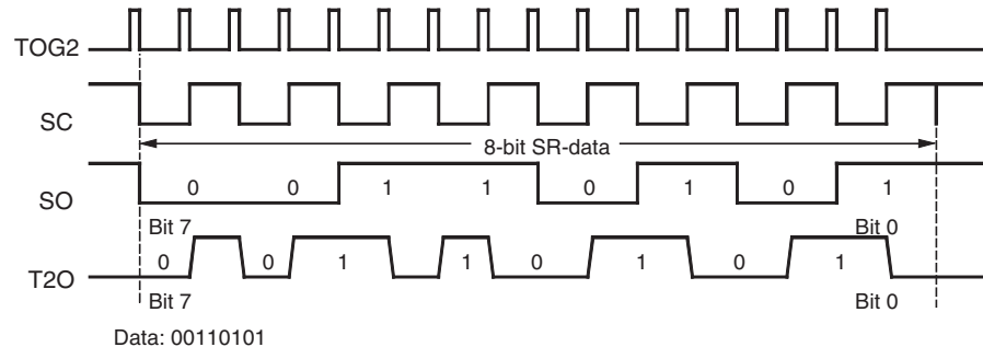
Figure 24-4. Manchester Modulation 1
