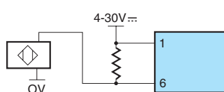
2-wire proximity sensor fast count input
